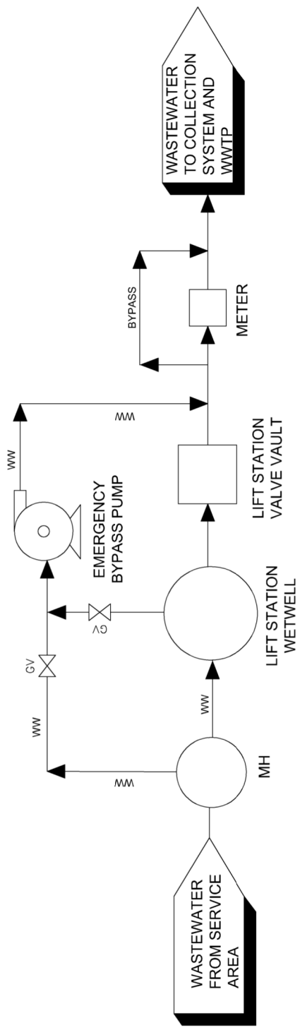
EMERGENCY LIFT STATION BACK UP PROCESS FLOW DIAGRAM
